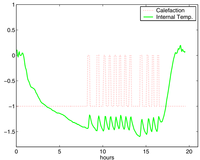
Fig. 2. Views of the historical data used for training: evolution of some normalized variables during three different time periods. On each plot the variable and its effect on the inside temperature of the greenhouse is shown.
