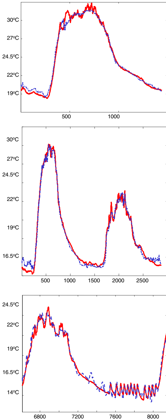
Fig. 3. Actual interior temperature (solid line) and simulation obtained by model NFIR^{12314} (dashed line) in a clear day (upper plot), in a day when ventilation was in use (middle plot) and in a day with heating (lowerplot). In all cases the horizontal scale is given in sampling periods (minutes).
